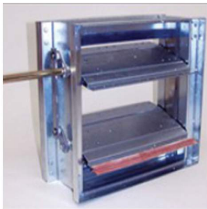
VCD: AIRFOIL
